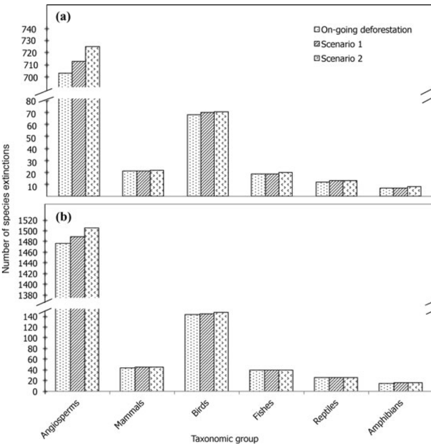
Figure 3. Projected number of species extinctions within taxonomic groups due to ongoing deforestation and forest loss due to dam building in the Indian Himalaya for species-area relations with a z value of 0.25 in (a) 2025 and (b) 2100 (scenario 1, dams built only in already-degraded forests; scenario 2, dams built haphazardly across the landscape including in dense forests). Predictions of extinctions are based on forest area data from Pandit et al. (2007).
