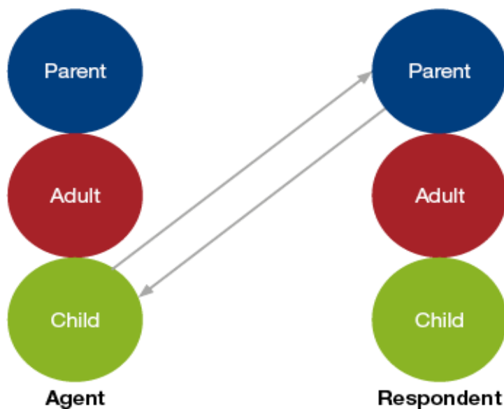
Fig. 5.7: Child-Parent transaction
